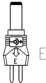
Hohlstecker/ hollowplug ø2,1xø5,5x12mm
